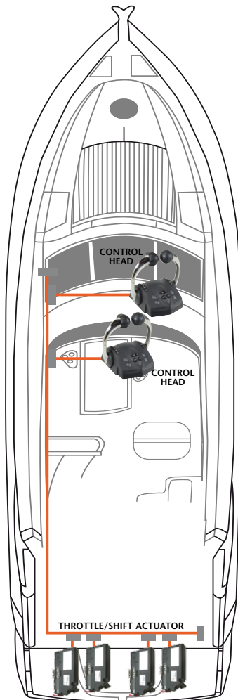
DUAL STATION / DUAL ENGINE
