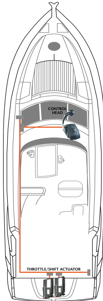
SINGLE STATION / SINGLE ENGINE
